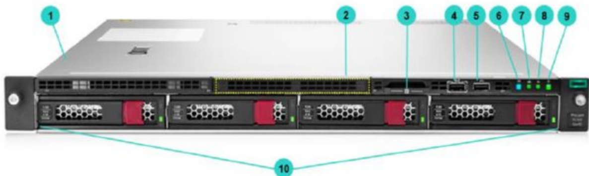
4 LFF chassis - Front View
